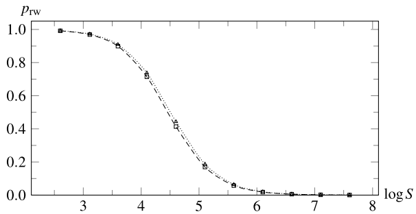
Fig. 3 Random walk encounter probability p_{rw} as a function of the (logarithmic) grain size for W/a = 10^{-5} , and for a type (a) (dashed/squares) or a type (b) (dotted/triangles) lattice, respectively
