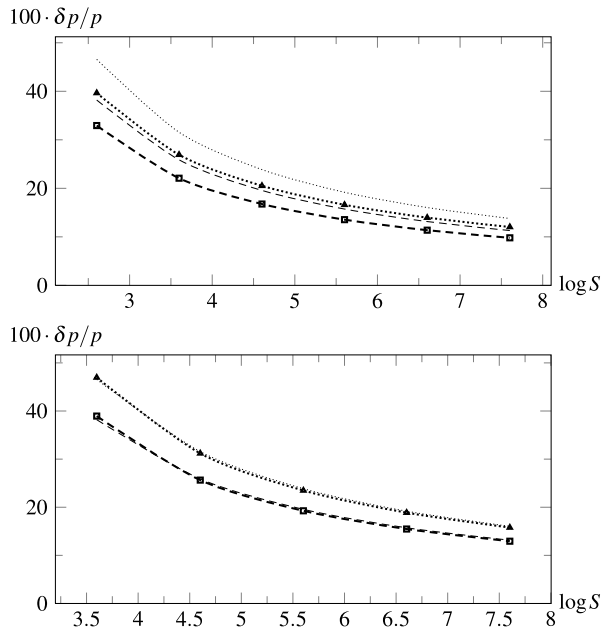
Fig. 2 Relative difference (in percent) of p_{\text{diff}} w.r.t. p_{\text{rw}} for SW/(4a) = 10^0 ( top , already a large lattice) and SW/(4a) = 10^1 ( bottom ), type (a) ( dashed/squares ), type (b) ( dotted/triangles ); thinner lines the prediction \Delta
