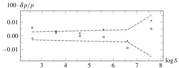
Fig. 6 Relative difference of \tilde{p}_{mc} w.r.t. \tilde{p}_{rw} for SW/(4a) = 10^{-4} , type (a) (dashed / squares), type (b) (dotted / triangles)
