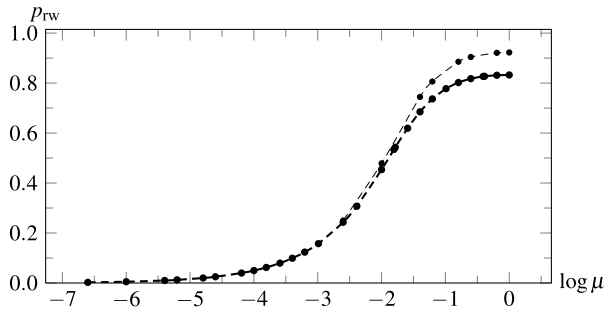
Fig. 4 Encounter probability (on a square lattice) as a function of \log \mu , for fixed sizes S = 4 \times 10^6 ( thick ) and S = 4 \times 10^2 ( thin ), respectively, and SW/(4a) = 10^{-2} in both cases
